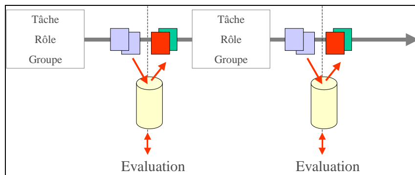
Figure 5 : CSCL Script.
