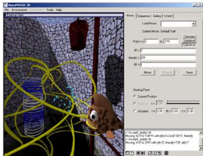
Figure 3 : Aquamoose.
